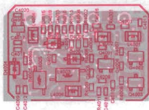
Component Side
