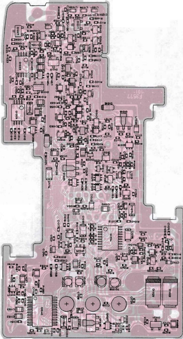
Chip Side
