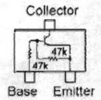
DTC144EU (26) (Q2007)
