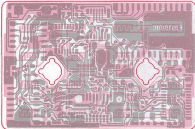
Keypad Side
