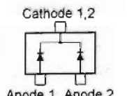
DAN222 (N) (D1001)
