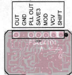
Connector Side
