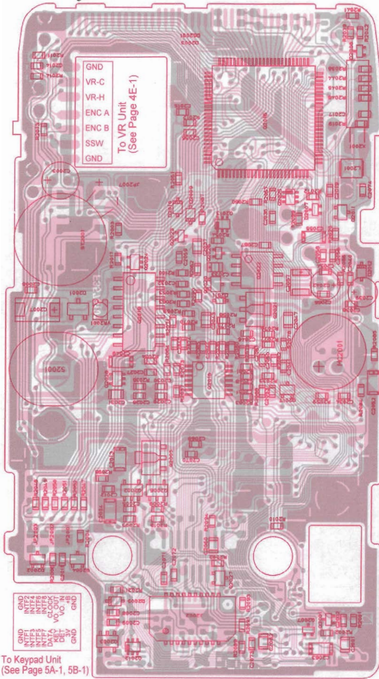
LCD Side
