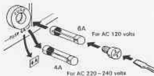
Fig. 3-1B Fuse replacement
