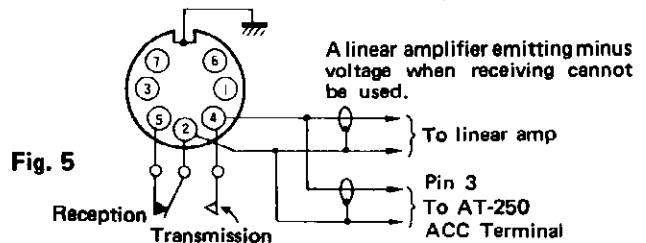
Rear view of the connector
