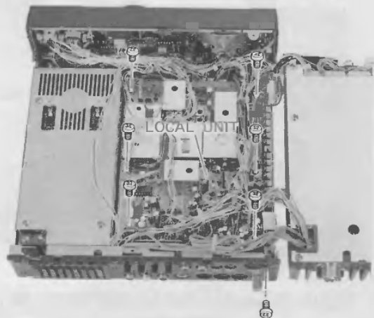
Figure 7: Local Unit Screws
