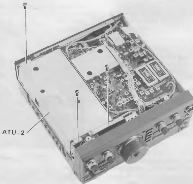
ATU-2 Mounting
