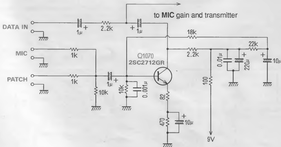
Transmitter AF Input Relationships
