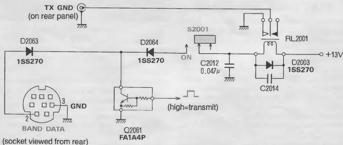
Linear Amp T/R Switching in the FT-890
