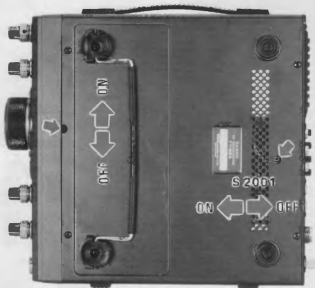
Switch Locations in Bottom Cover
